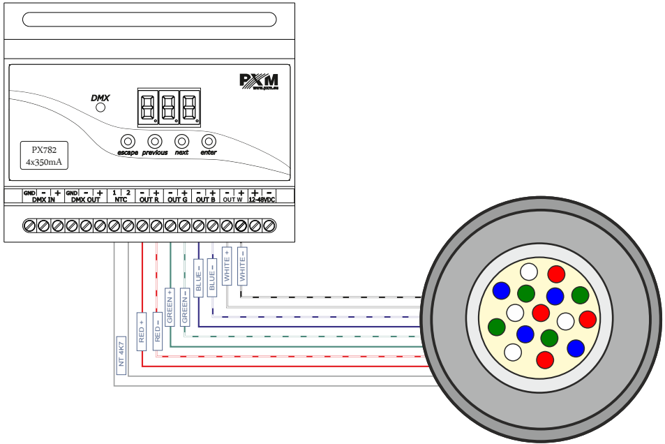
RGBW lamp with built-in NTC 4K7 thermistor
